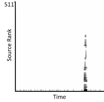
Figure 3: Source rank distribution over time observed from rank zero in SMG2000 with 512 processes.
